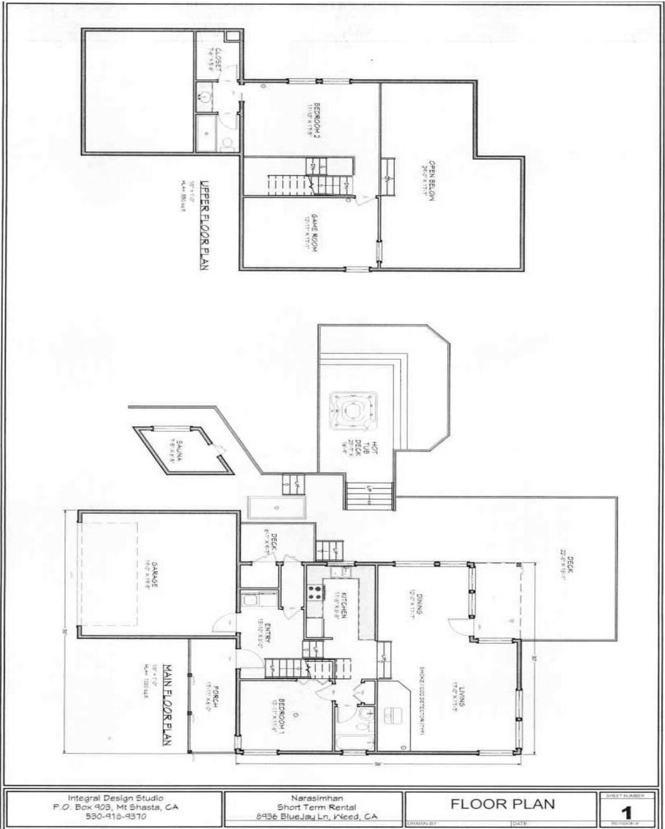
Figure 4: Floor Plan
